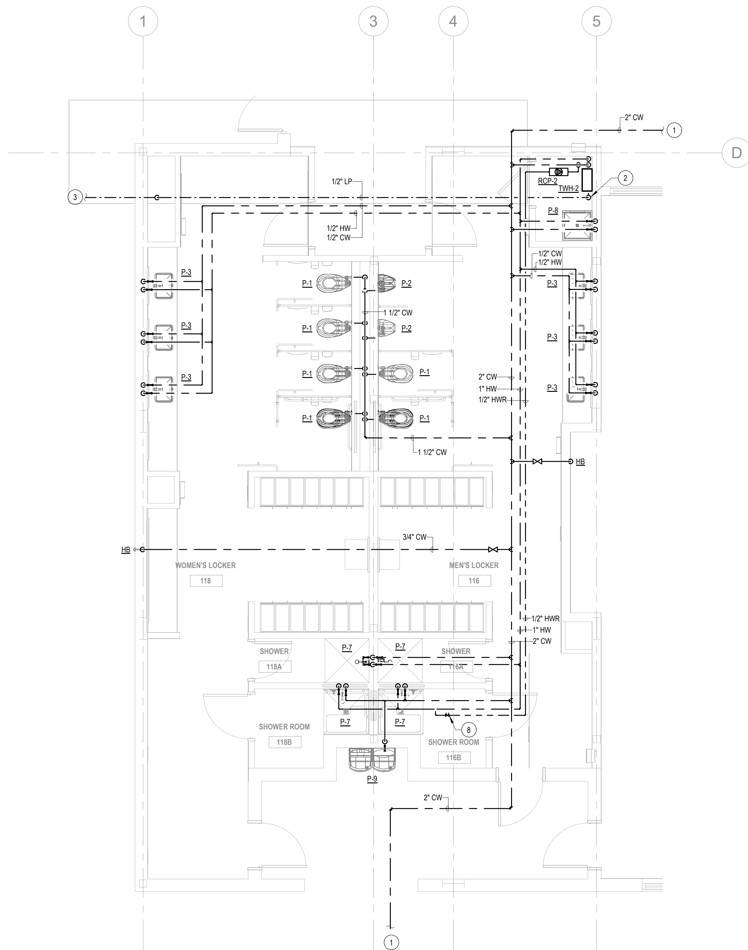
1 DOMESTIC WATER AND GAS - ELNARGED PLAN - LOCKER ROOMS 1/4" = 1'-0"
