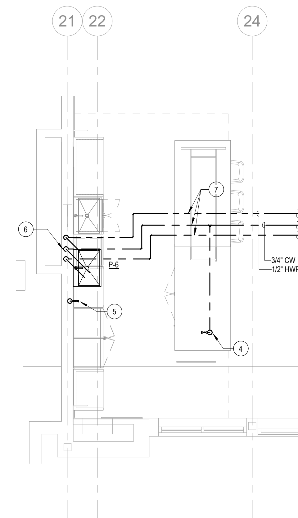
3 DOMESTIC WATER AND GAS - ENLARGED PLAN - BAR 1/4" = 1'-0"
