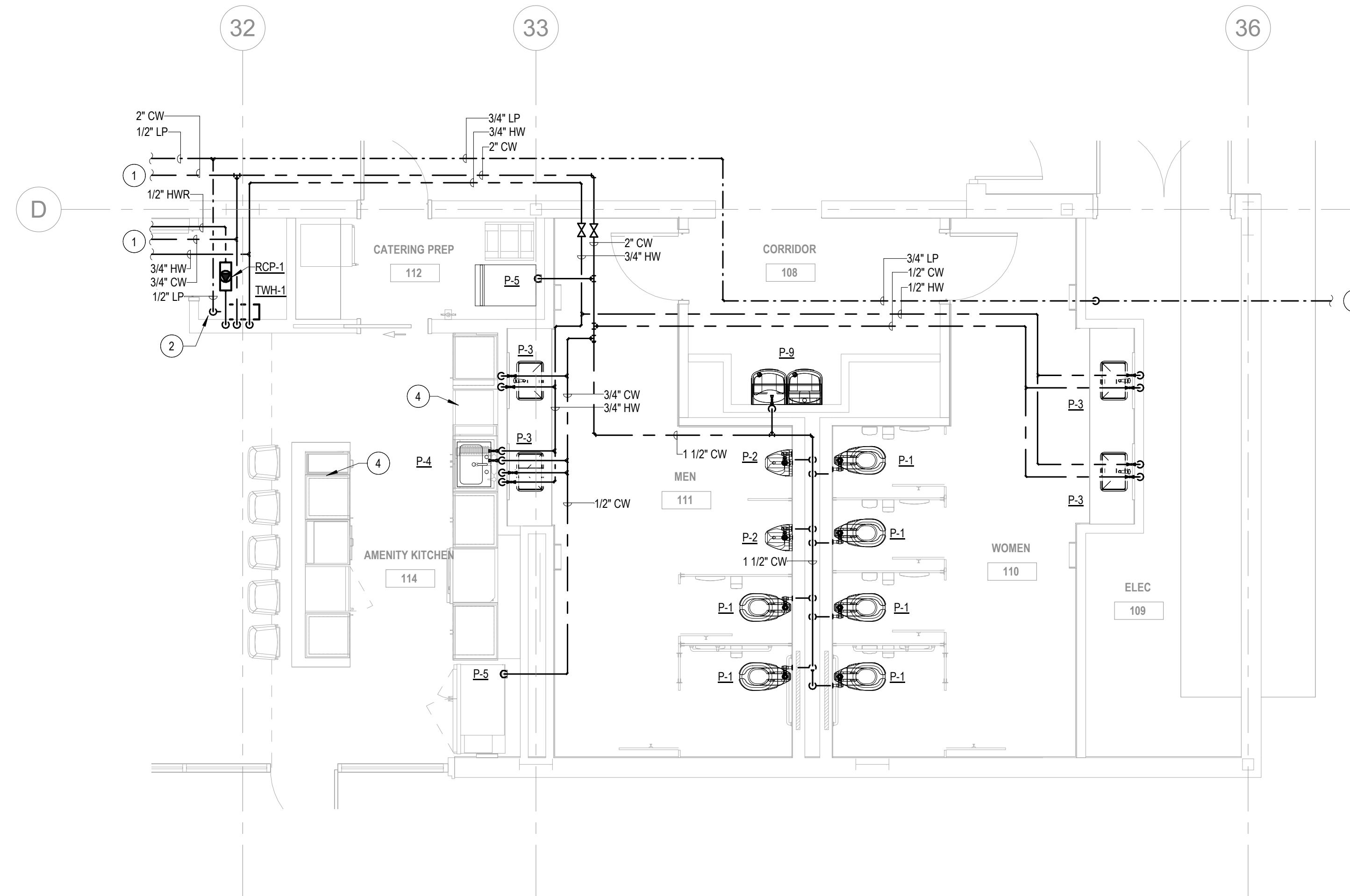
2 DOMESTIC WATER AND GAS - ENLARGED PLAN - RESTROOMS 1/4" = 1'-0"
