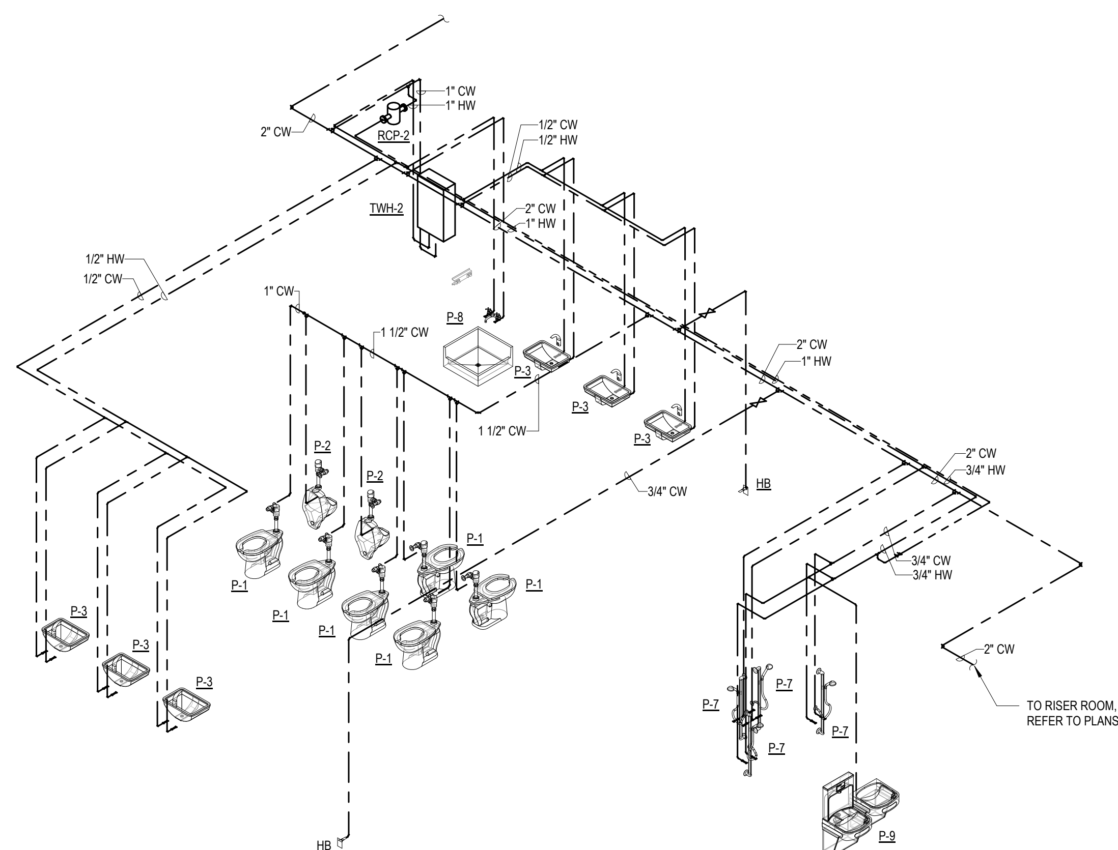
4 DOMESTIC WATER ISOMETRIC - LOCKER ROOMS
