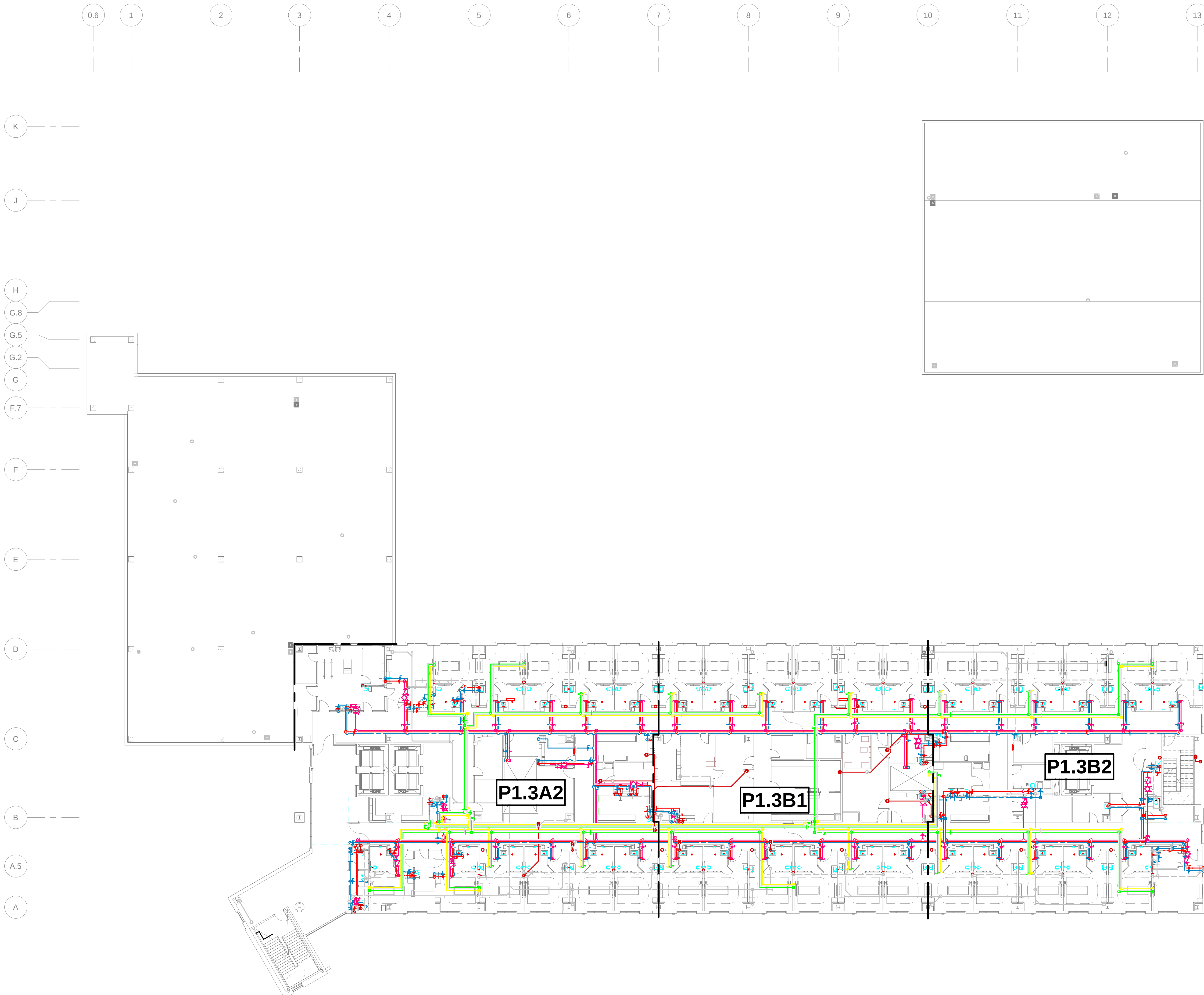
LEVEL 3 COMPOSITE PLUMBING PLAN 1/8" = 1'-0"
