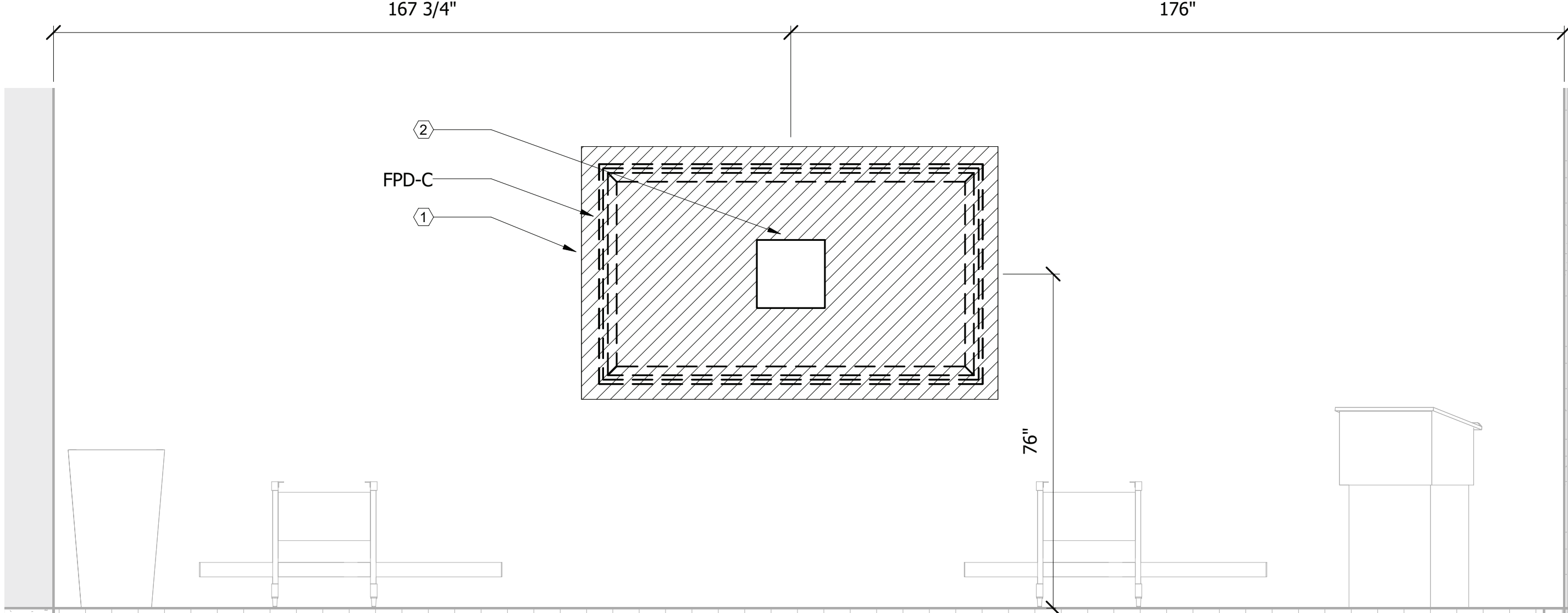
SIMULATION CLASSROOM 200B SCALE: 1/2" = 1'-0"
