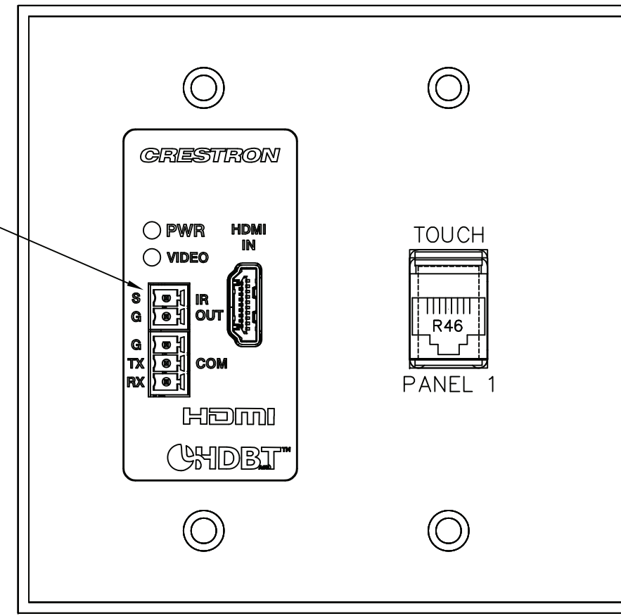
3 TWO GANG FACE PLATE Scale: NTS
