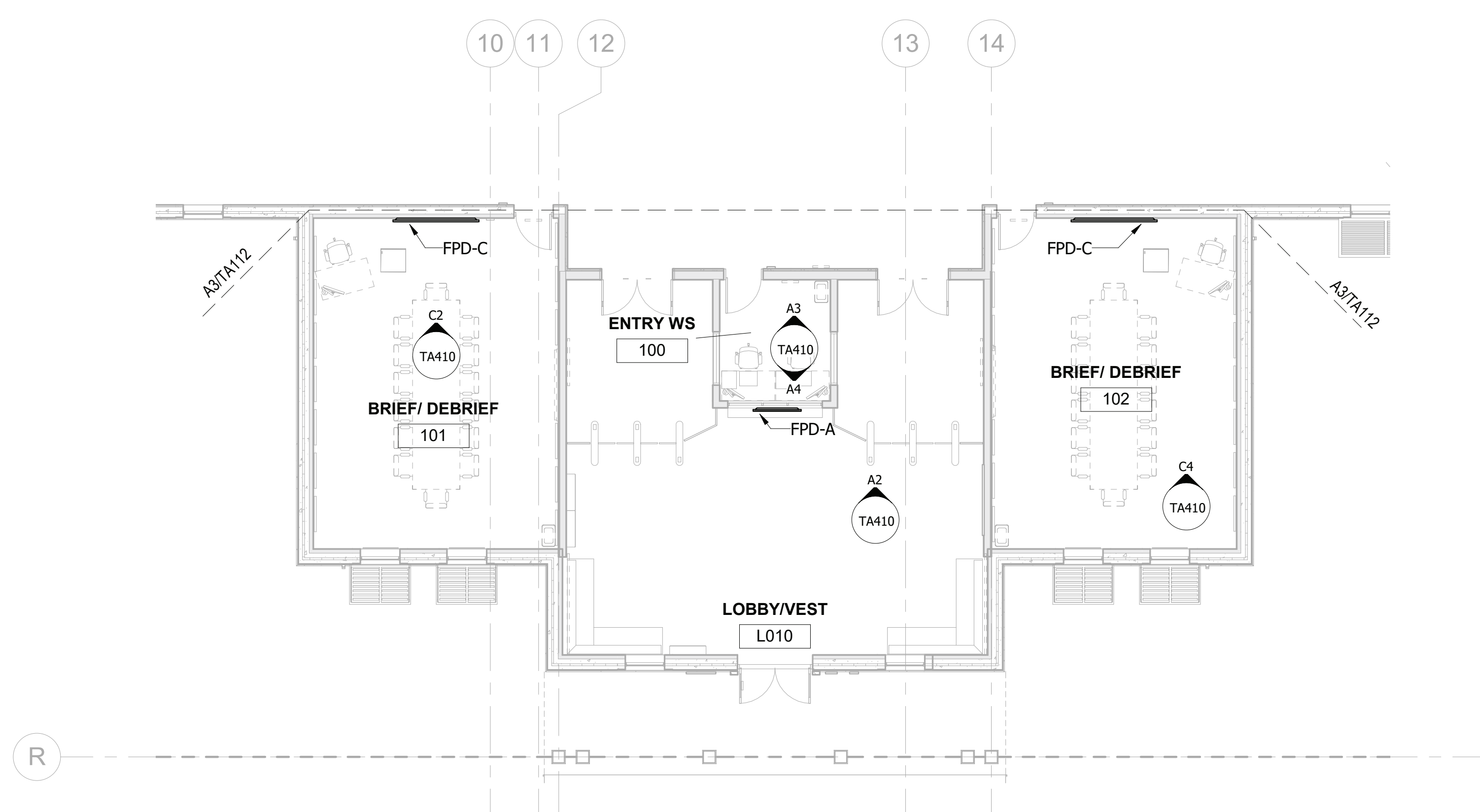
EQUIPMENT - FLOOR PLAN - AREA D SCALE: 1/8" = 1'-0"
