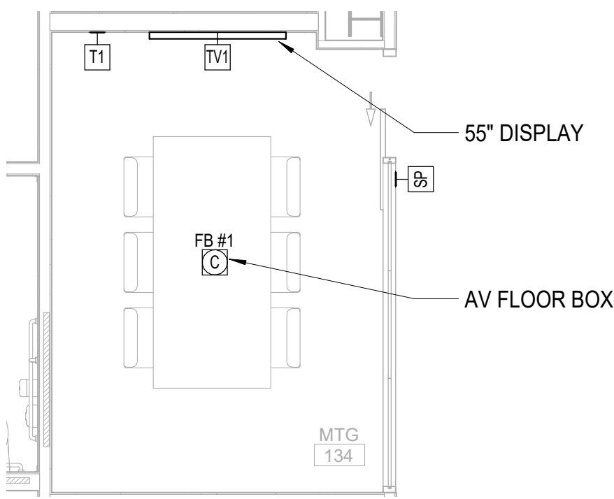
2 AV TYPICAL LEVEL 1 MEETING ROOM - ENLARGED PLAN AV-201 1/4" = 1'-0"
