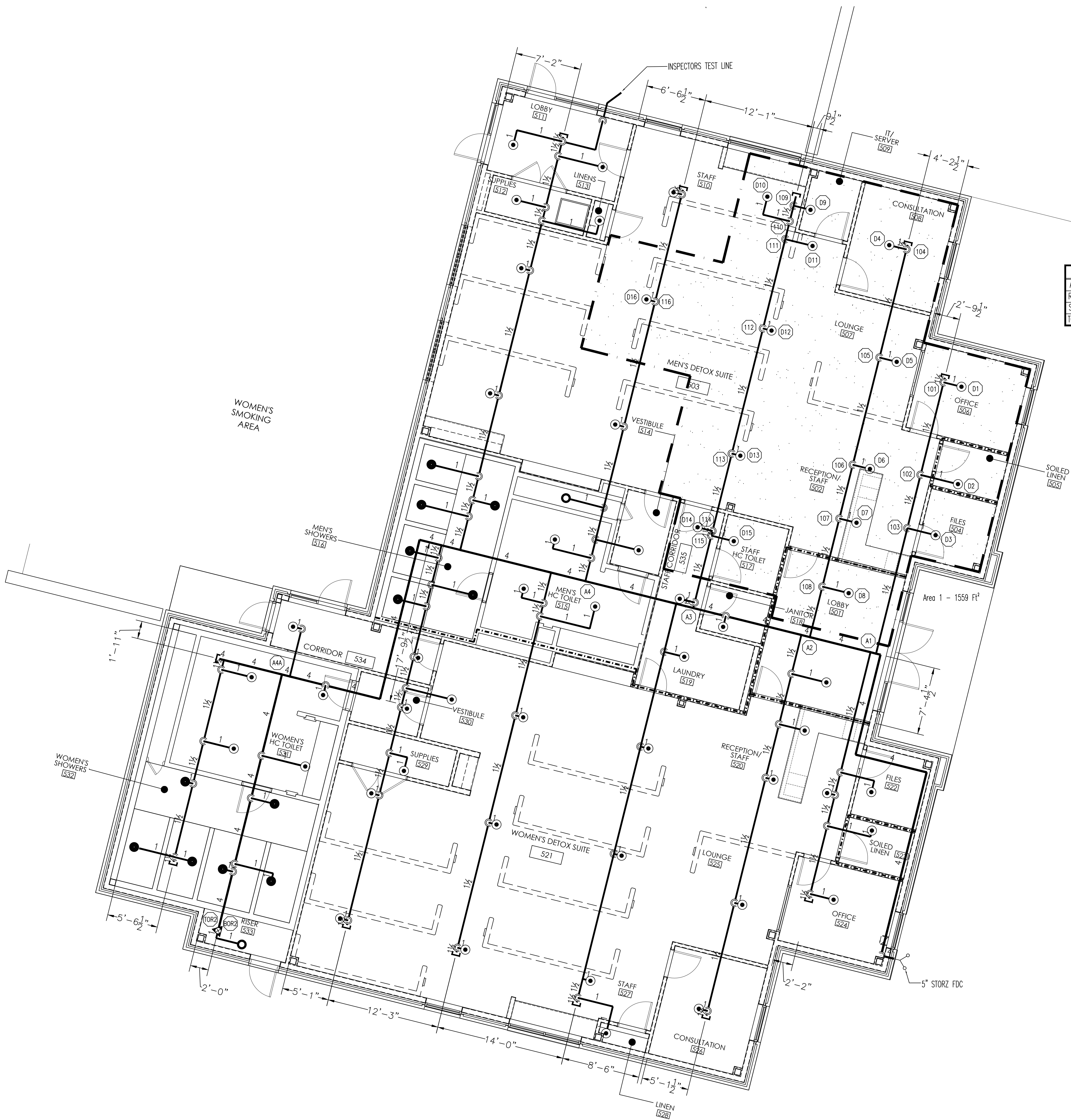
1 DETOX BUILDING - PIPING PLAN FP 11 \frac{3}{16}'' = 1'-0''
