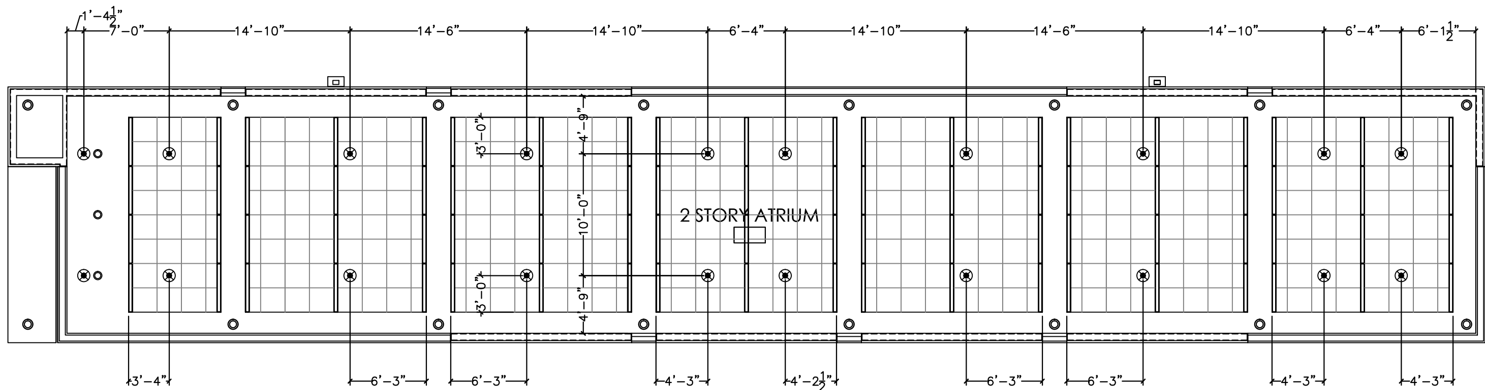
2 ADMIN. BUILDING - ATRIUM RCP FP 4 1/8" = 1'-0"
