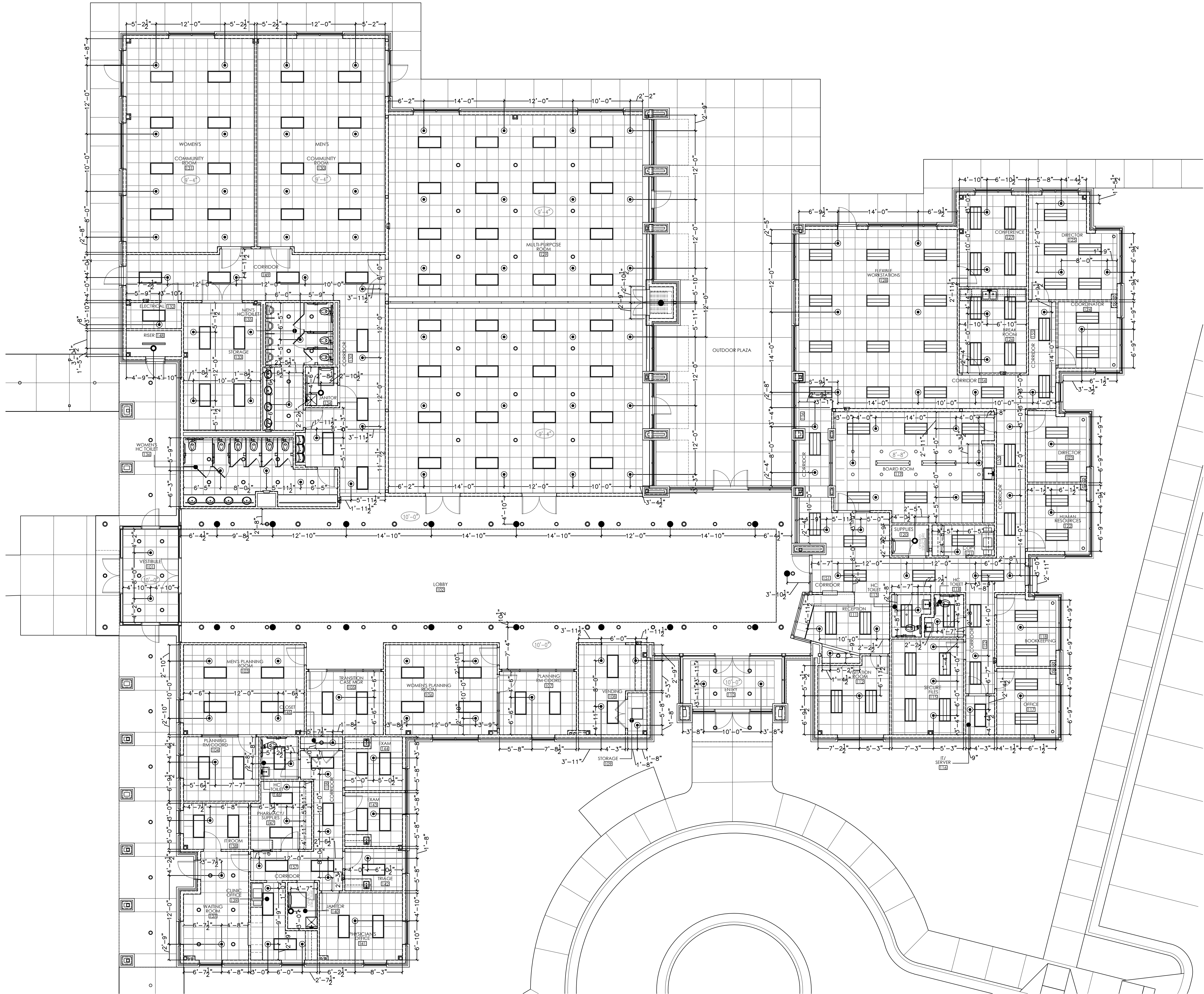
1 ADMIN. BUILDING - RCP FP 4 1/8" = 1'-0"
