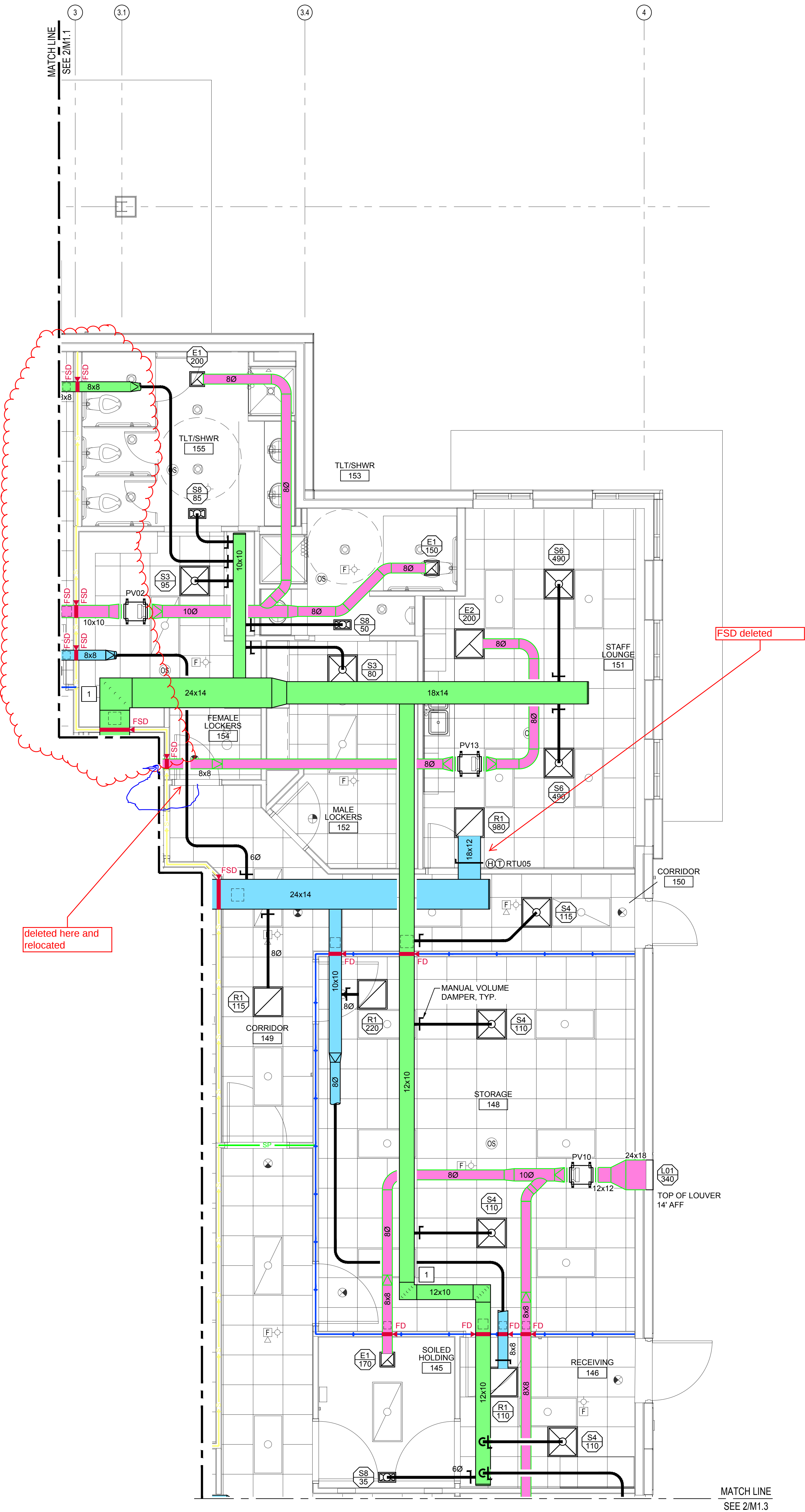
2 FLOOR PLAN 1/4" = 1'-0"
