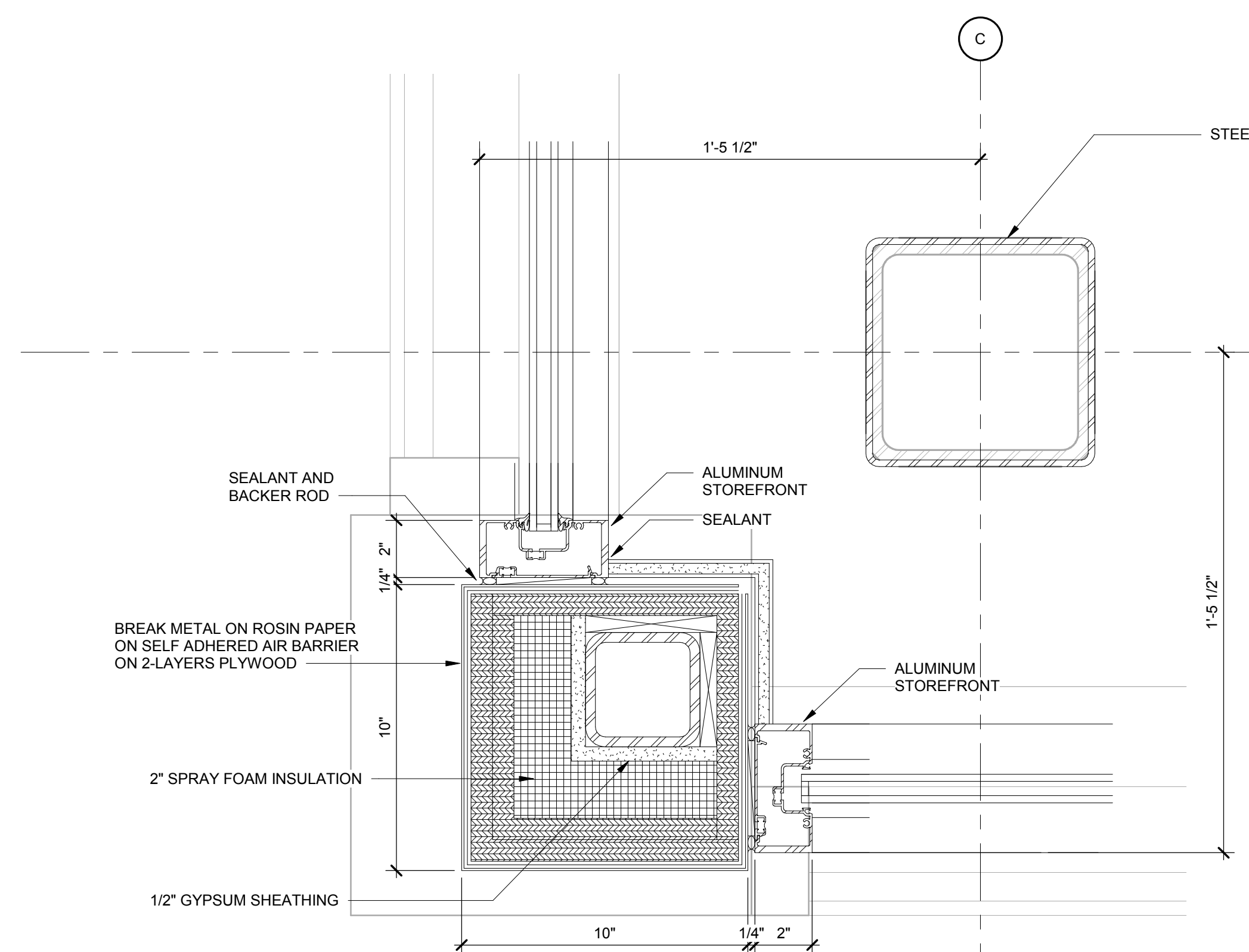
DINING STOREFRONT PLAN DETAIL ALONG B (F1) 3" = 1'-0"
