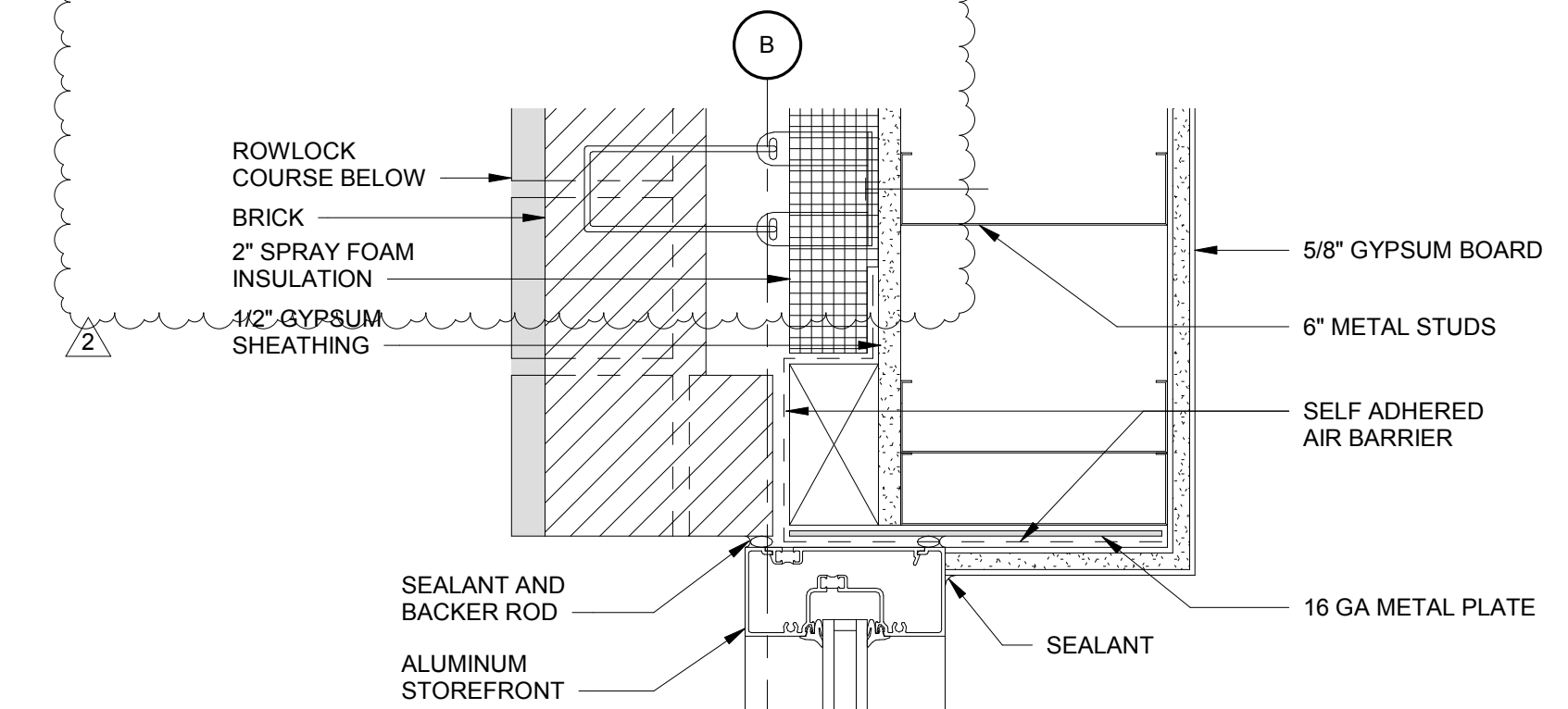
DINING STOREFRONT PLAN DETAIL ALONG B (F1) 3" = 1'-0"
